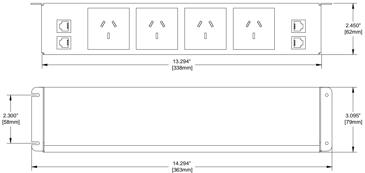
Diagram 11: UT240-511 Australia
