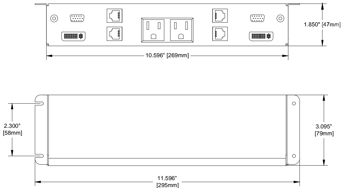
Diagram 5: UT240-313 U.S./Canada
