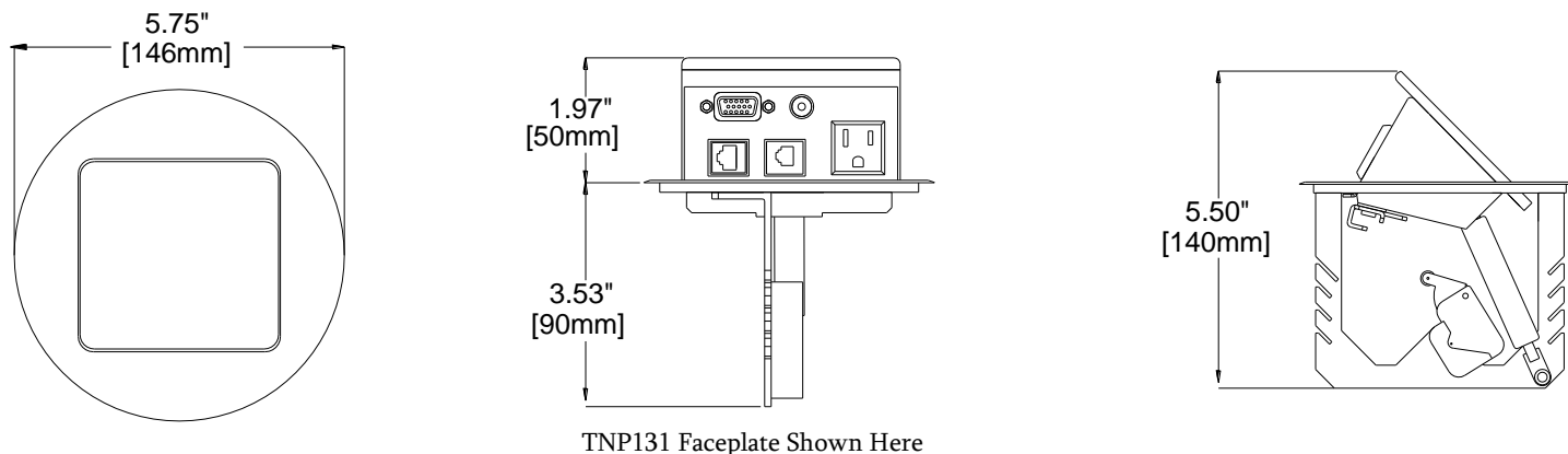
Diagram 1: Round Bezel Dimensions (TNP126, TNP131, TNP141 - includes models ending in C & S)
