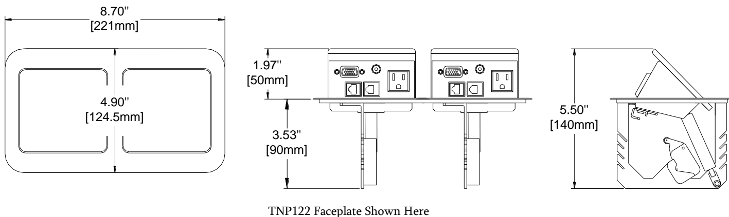
Diagram 3: Dual Unit Dimensions (TNP122, TNP142 - includes models ending in C & S)
