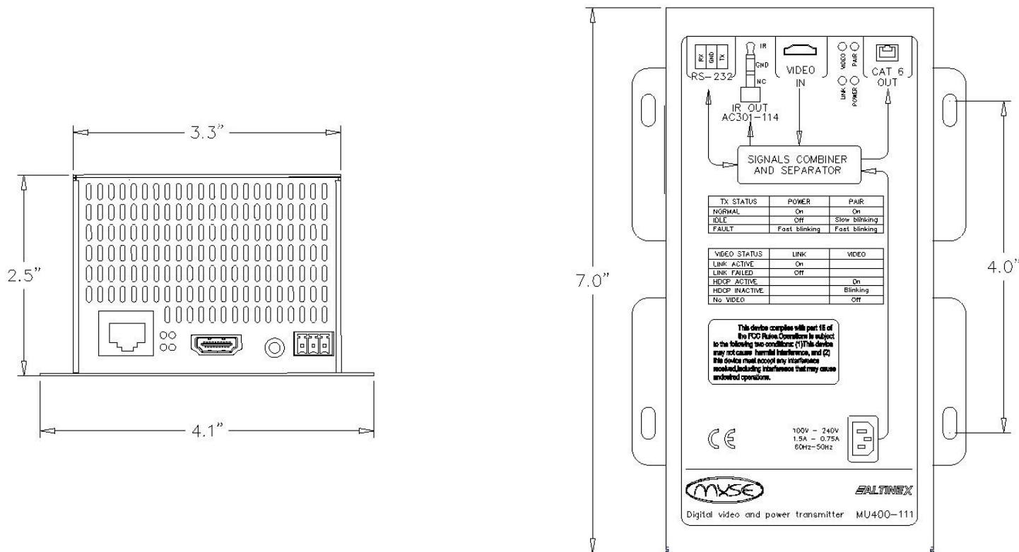
Diagram 3: Transmitter Dimensions
