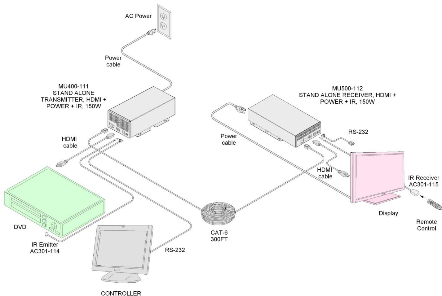
Diagram 2: Typical Setup
