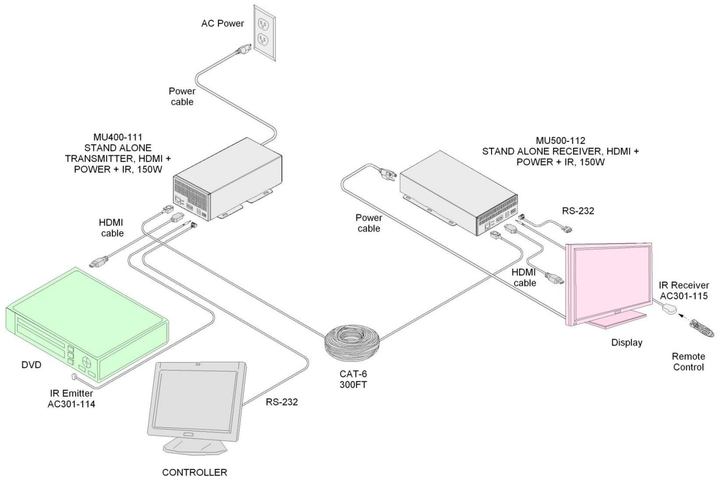
Diagram 1: Typical Setup
