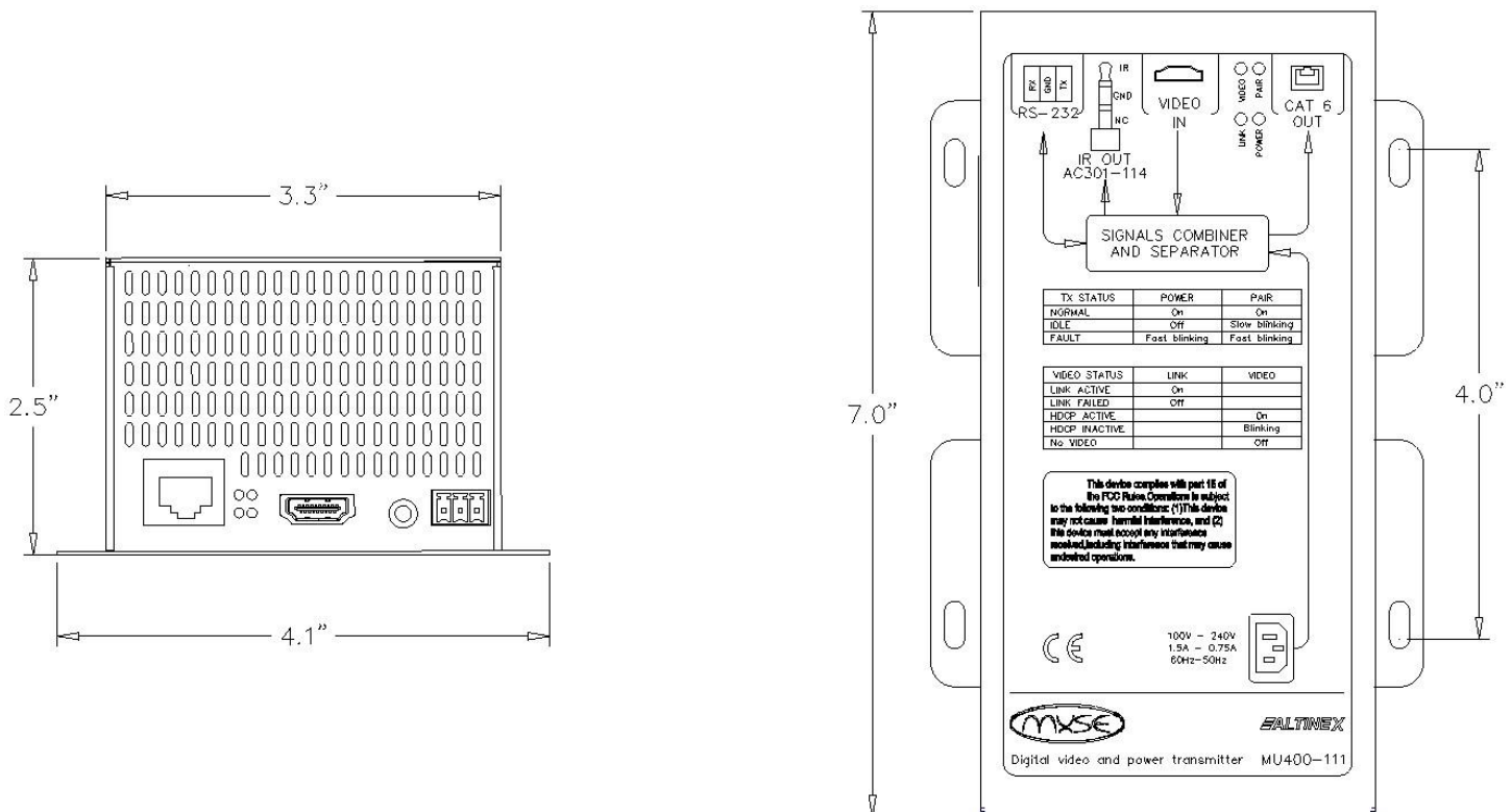
Diagram 3: Transmitter Dimensions
