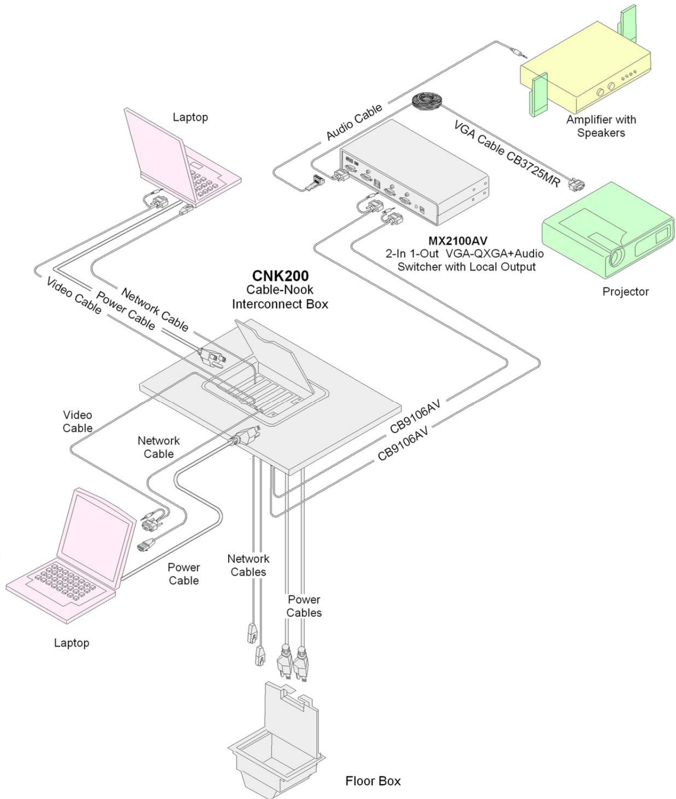
Diagram 1: Typical Setup
